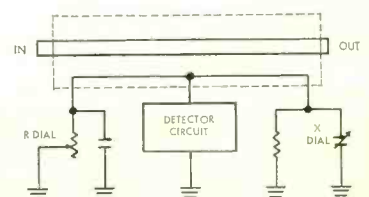
Fig. 3. Simplified schematic of the input to the matching section and final OIB.
