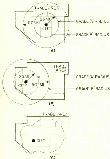
Fig. 1. A directional antenna (C) will cover (with similar ERP) the market area as well as a centrally located omnidirectional antenna (A).
