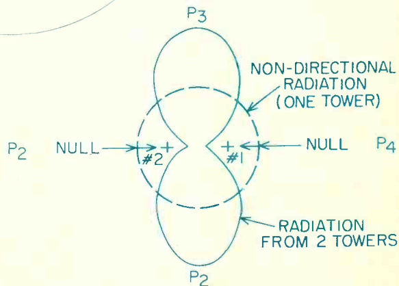
Fig. 4. Radiation of array in Fig. 3.
