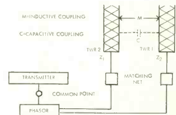
Fig. 1. Diagram of 2-tower antenna network.
